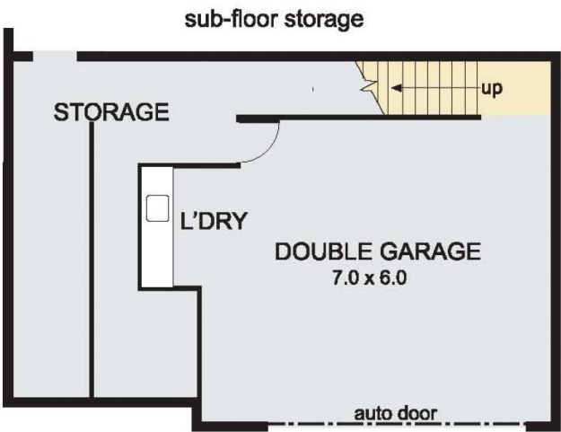
LOWER FLOOR
