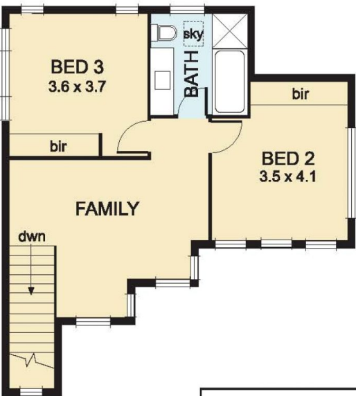
UPPER FLOOR
